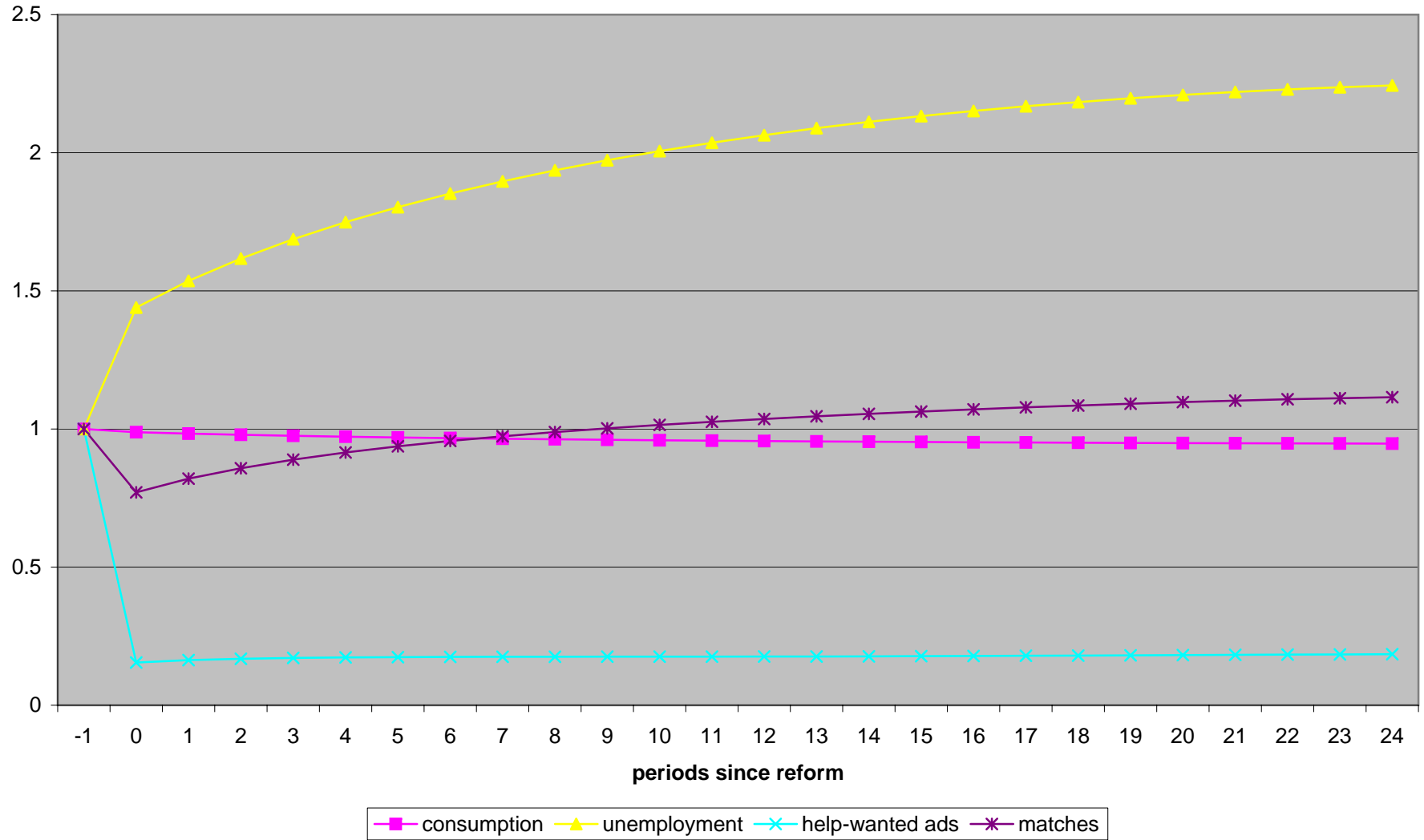
FIGURE 1 Transitory dynamics (linear preferences)
