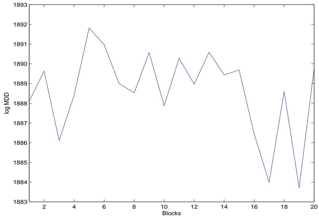
FIGURE 3. The 3 variance-only (3v) model with the standard MHM method.
