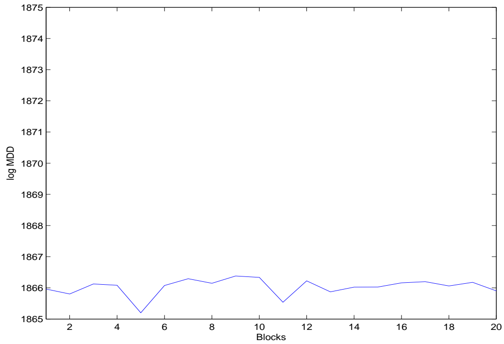
FIGURE 2. The 3 variance-only (3v) model with the new MHM method.
