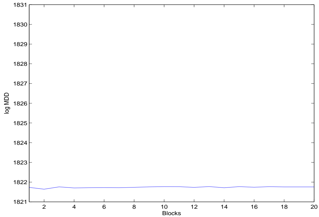
FIGURE 1. The 2-regime variance-only ( 2v ) model with the new MHM method.
